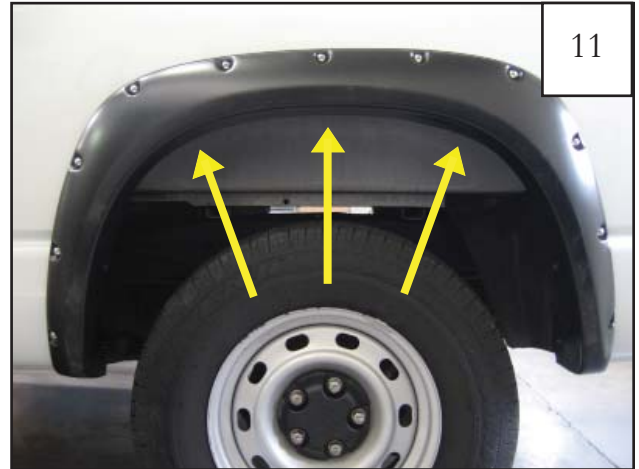
11 Hold flare in place and mark three locations with a grease pencil using the holes in the flare as a guide. See step 12 & 13.
