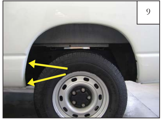
9 Install Clip (CL1-0011) in these locations. See step 10.
