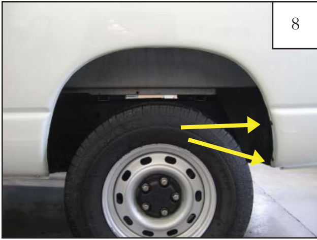
8 Remove two factory installed screws using an 8 mm socket wrench. Keep screws for installation of the rear flare.
