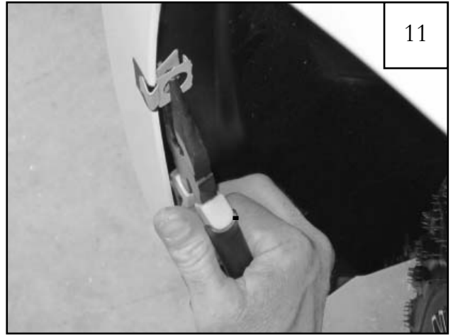
Using needle nose pliers, snap clip together to secure to the vehicle.
