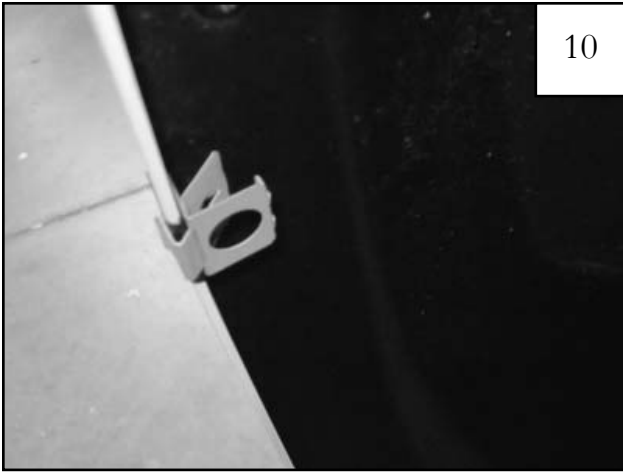
Center clips on the tabs installed in Step 8 and push onto the bumper cover.
