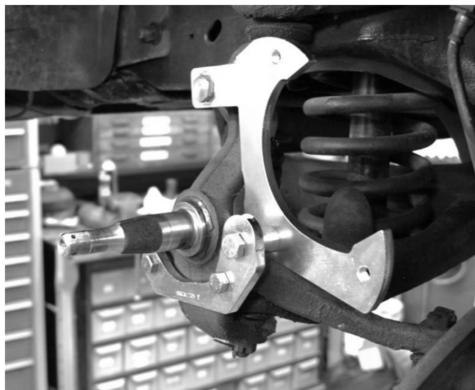
Figure 3 – Secondary Caliper Mounting Bracket Installed
