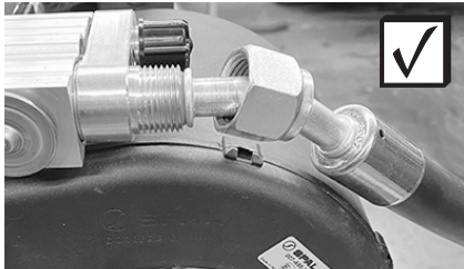
Properly Seated O-ring Land
