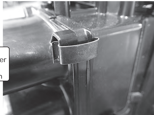
Spring Clip Installed
